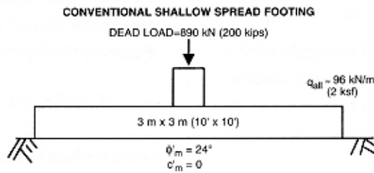
Figure 5a. Sliding Resistance Example for Footing Supported by Unreinforced Soil.
